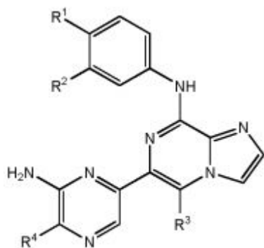
Formel I
