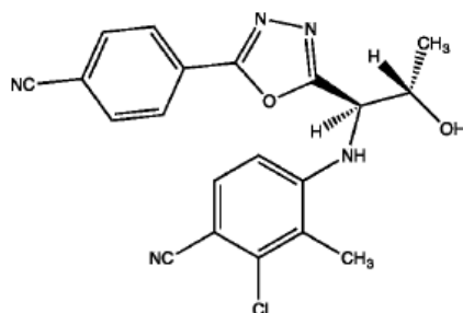
RAD140 (Compound III)
