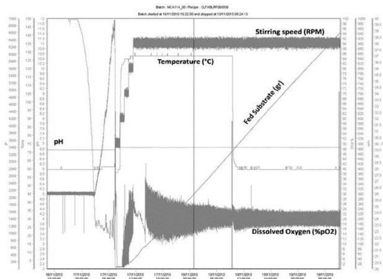
Слика 1: A typical fermentation profile with the High Cell Density Induction (HCDI) processes and the parameters monitored during 20L-scale fed-batch fermentation.
