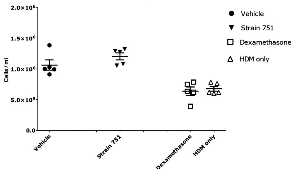
FIG. 1 Total cell counts.
