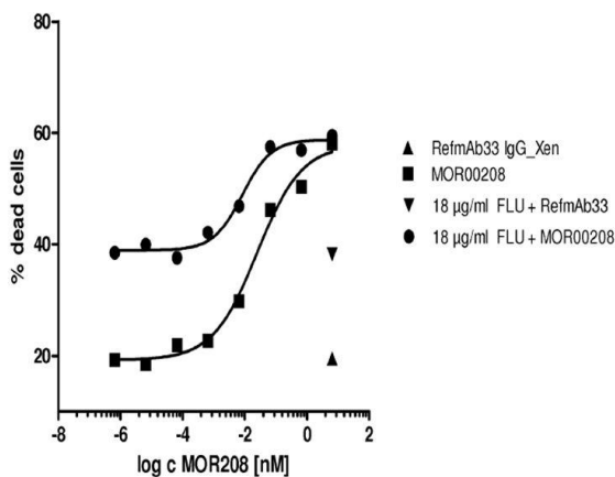
Figure 1 Слика 1 Cytotoxicity of MOR208 and FLU alone and in combination
