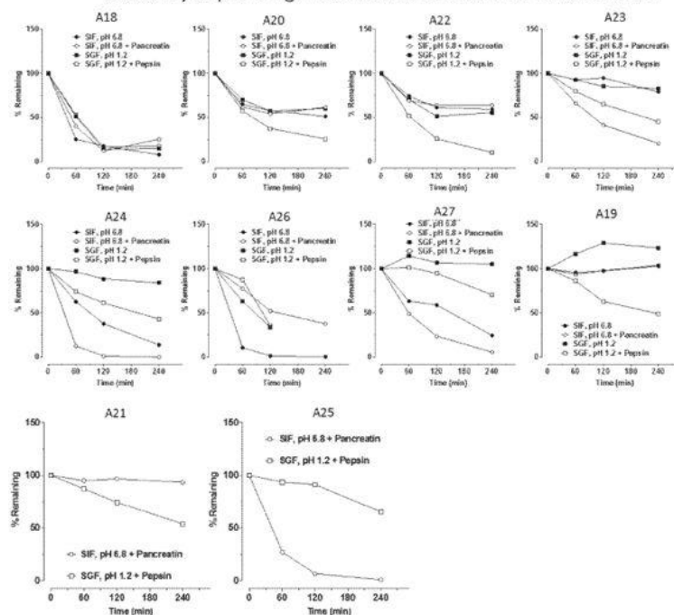
Сл.1 .. Stability of pro-drugs in Simulated Intestinal or Gastric Fluids
