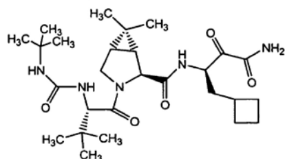
Formula Ic;
