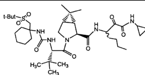
Formula IIa;
