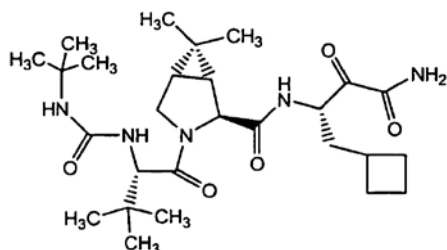
Formula Ib;
