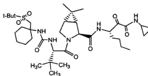
Formula IIb;
