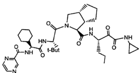
Formula III;
